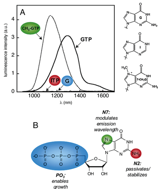
Figure 2. Effect of specific chemical functionalities present on GTP on PbS quantum dot synthesis. (A) Luminescence spectra obtained when GTP, G, ITP, and 7-CH 3 -GTP were used for PbS synthesis. (B) Proposed roles of phosphate and base functionalities on GTP in nanoparticle nucleation, growth, termination, stabilization, and passivation.
