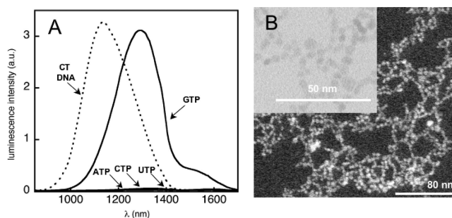
Figure 1. Effect of varying the nucleotide on the results of PbS nanocrystal synthesis. (A) Photoluminescence spectra under 633 nm, 3.3 mW excitation from a HeNe laser. The use of GTP ligand results in strongly luminescent, stably dispersed nanocrystals. In the presence of ATP, CTP, and UTP, syntheses produced mainly precipitate. CT DNA produces a strong luminescence spectrum that is narrower than and blue-shifted relative to GTP–NCs. (B) TEM of PbS quantum dots synthesized in the presence of GTP.
